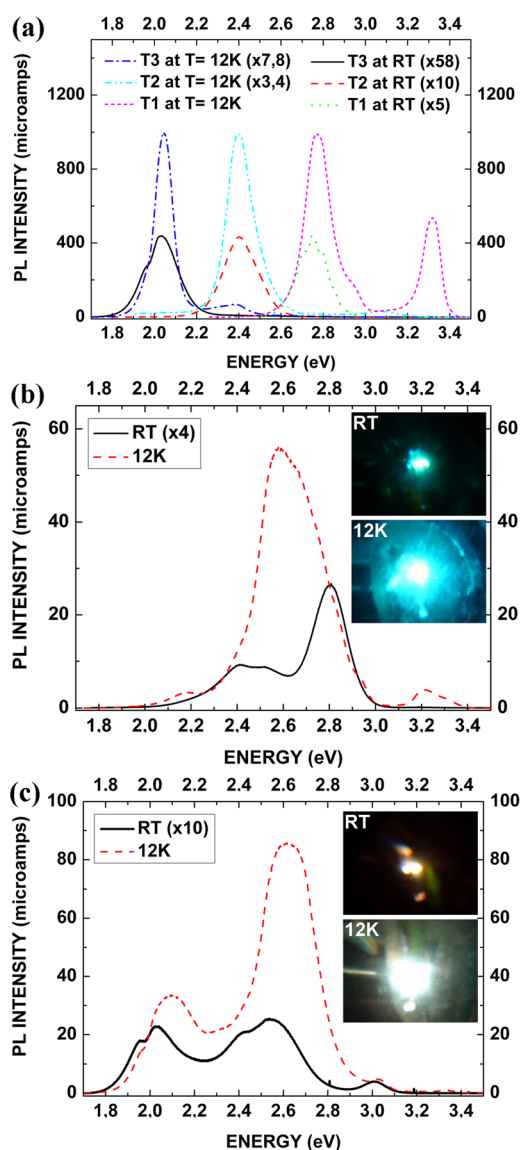
FIG. 2. Room- and low temperature (12 K) PL spectra of (a) samples T1, T2, and T3, (b) T4, and (c) T5 (insets show photographs of the emission color taken during the PL experiments; numbers in brackets correspond to the magnification factor of the respective spectrum).
